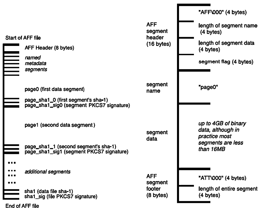
Fig. 2 – AFF file structure (left), AFF segment structure (right) (Garfinkel, 2006).
