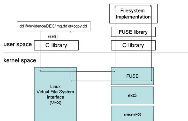
Fig. 4 – FUSE architecture.
