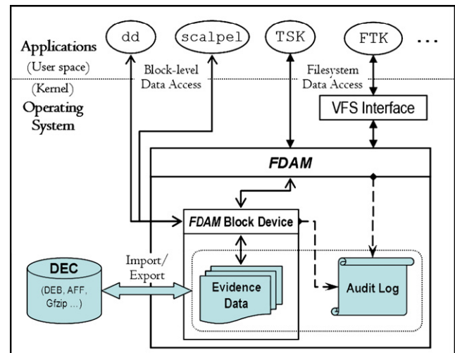
Fig. 3 – Forensic discovery auditing module (FDAM): architectural diagram.
