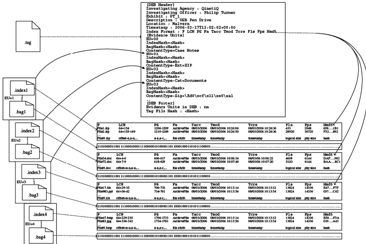
Fig. 1 – An example of Digital Evidence Bag (DEB) (Turner, 2006).
